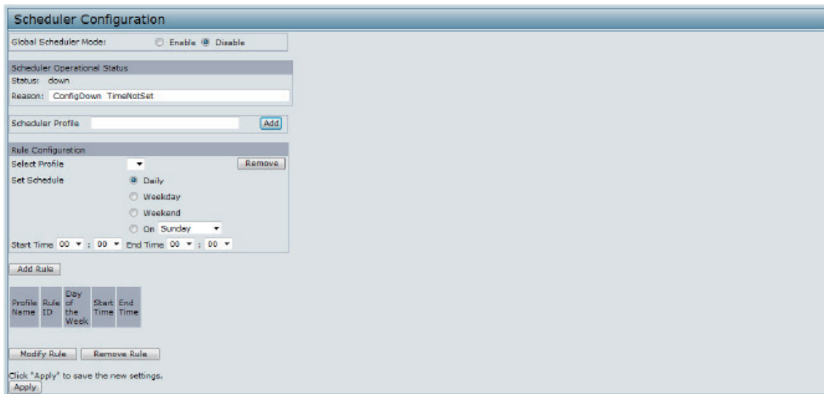
Figure 21 - Scheduler Configuration
