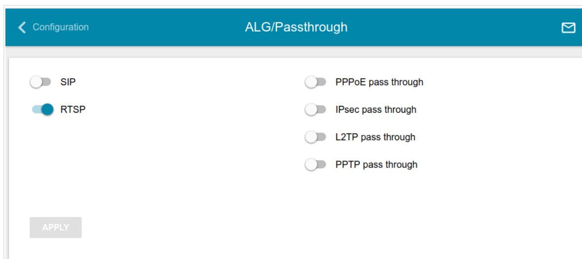
Figure 118. The Advanced / ALG/Passthrough page.
