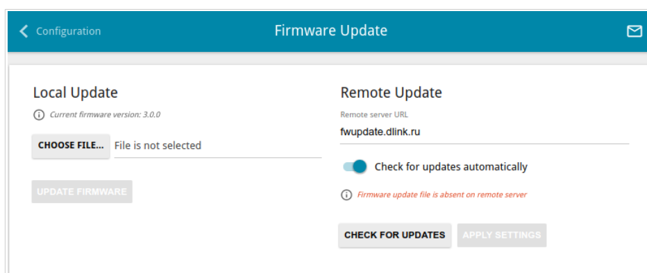
Figure 133. The System / Firmware Update page.
