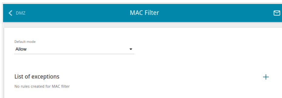
Figure 128. The Firewall / MAC Filter page.
