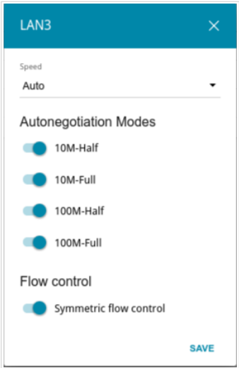
Figure 105. The window for changing the settings of the router's port.
