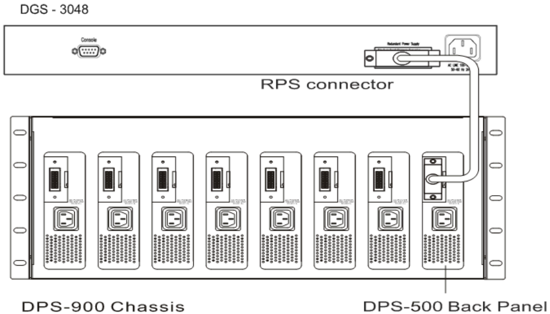
Figure 2-3. DPS-500 in DPS-900 Case with DGS-3048
