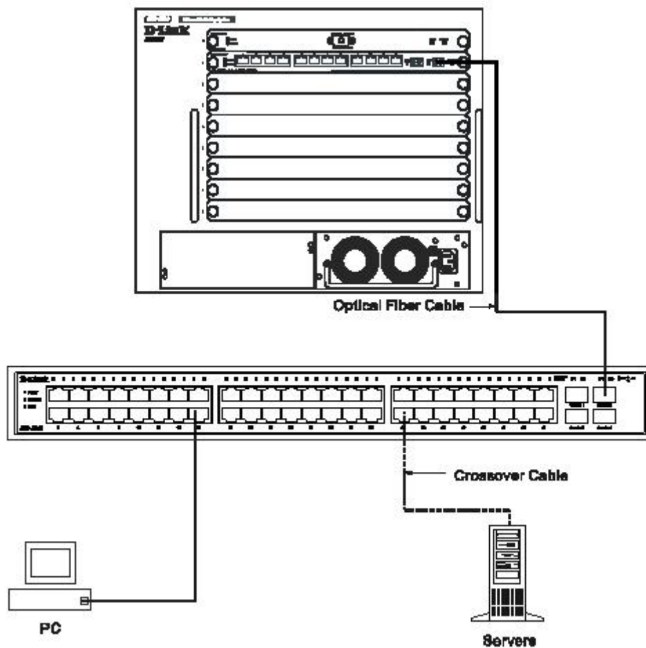
Figure 4-3 Switch Connected by an Optical Fiber Cable to a Core Router Switch, with a Server Connected by Crossover Cable and a PC Connected by a Category 3, 4, 5, or 5e UTP/STP cable
