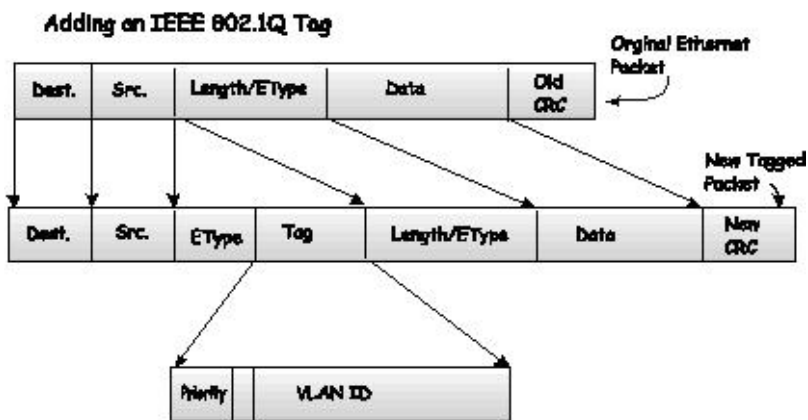
Figure 8- 3. Adding an IEEE 802.1Q Tag
