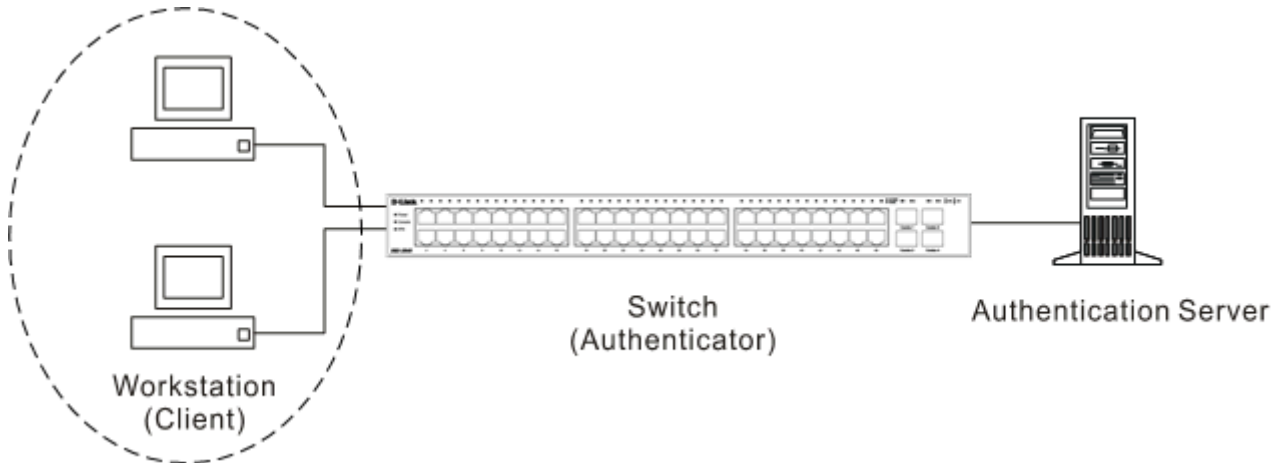
Figure 10- 5. Client
