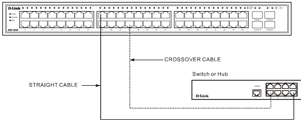
Figure 4-2. Switch Connected to a Normal (non-Uplink) Port on a Hub or Switch Using a Straight or Crossover Cable
