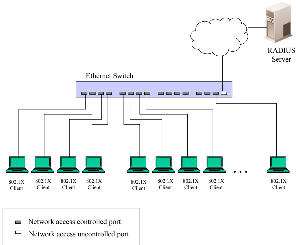
Figure 10- 6. Example of Typical Port-Based Configuration
