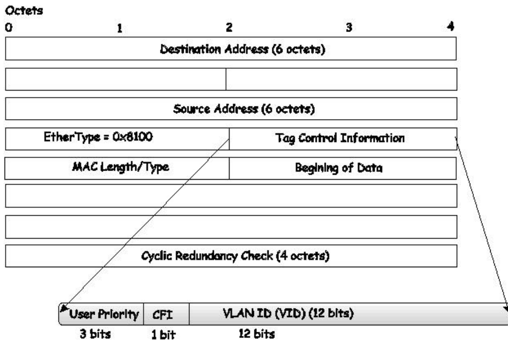
Figure 8- 2. IEEE 802.1Q Tag
