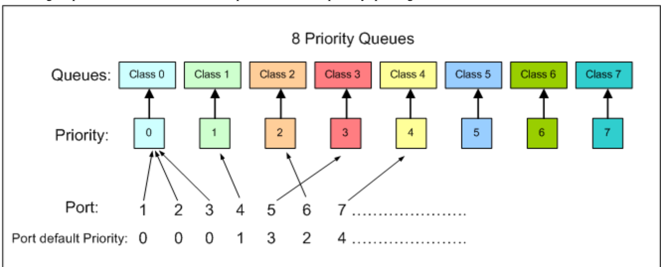
Figure 9- 1. Mapping QoS on the Switch
