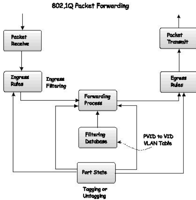
Figure 8- 1. IEEE 802.1Q Packet Forwarding
