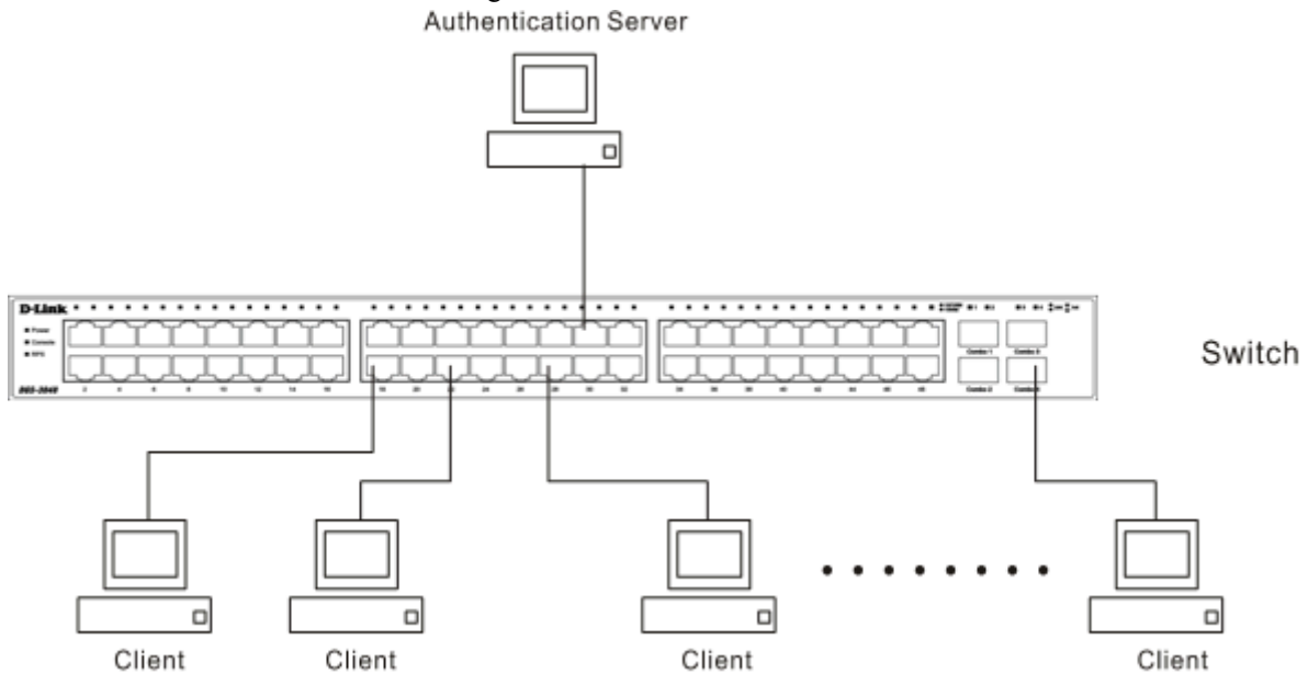
Figure 10- 3. Authentication Server
