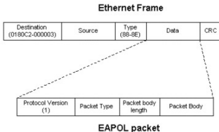
Figure 10- 1. EAPOL Packet
