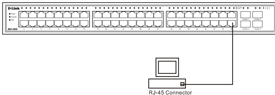
Figure 4-1. Switch Connected to an End Node
