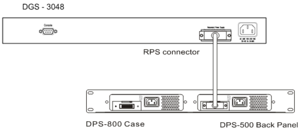
Figure 2-4. DPS-500 in DPS-800 Case with DGS-3048
