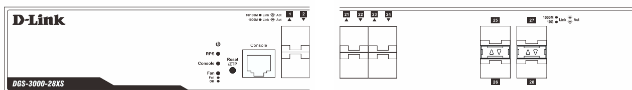
Figure 1-16 LED indicators for a DGS-3000-28XS Switch
