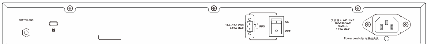
Figure 1-23 Rear panel view of a DGS-3000-28X Switch
