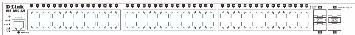
Figure 1-8 Front panel view of a DGS-3000-52L Switch
