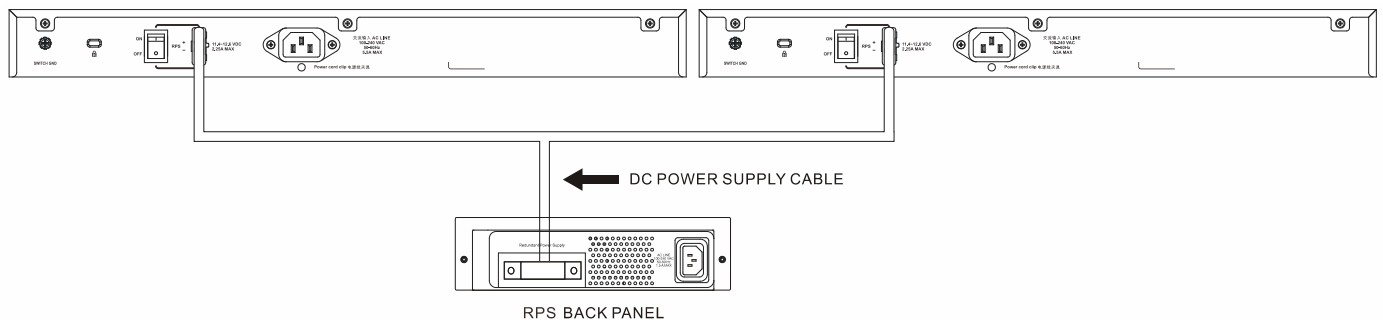
Figure 2-11 Connecting two Switches to the RPS
