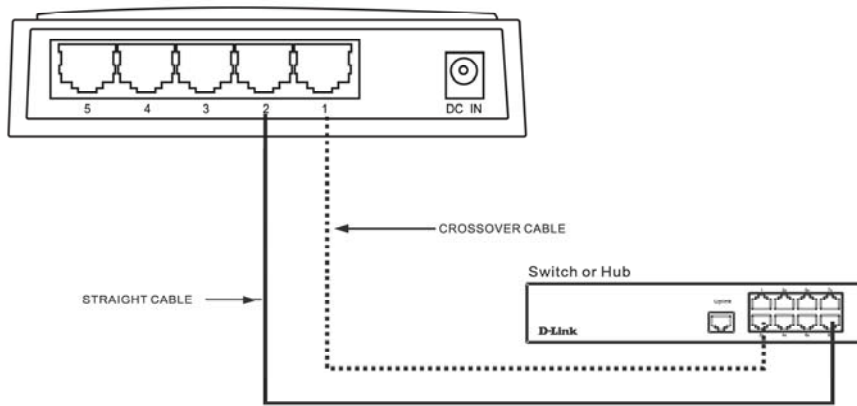
Figure 3-2. Switch connected to a port on a hub or switch using either a straight or crossover cable—any standard Ethernet cable is fine
