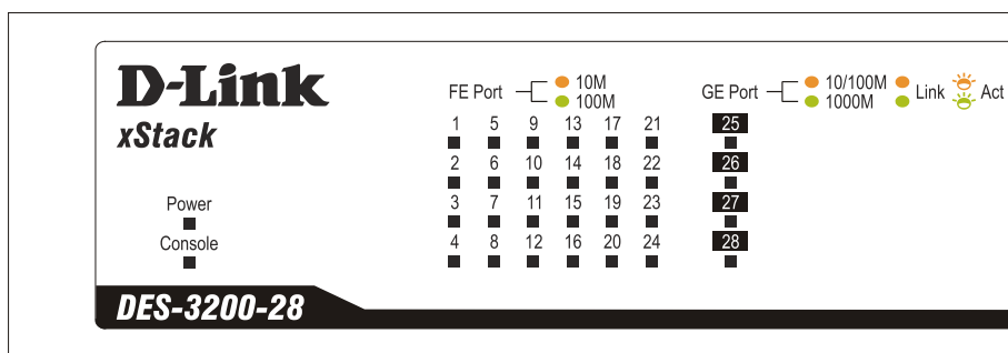
Figure 1- 3. LED Indicators on DES-3200-28 Switch
