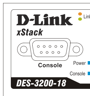
Figure 1- 2. LED Indicators on DES-3200-18 Switch
