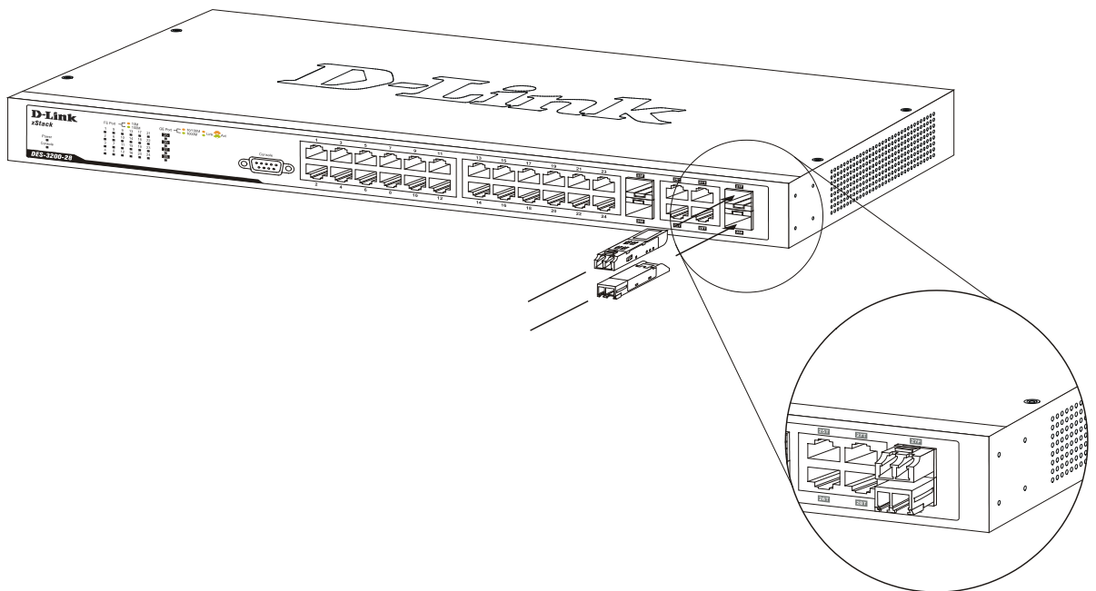
Figure 1- 16. Inserting the Mini-GBIC modules into the Switch
