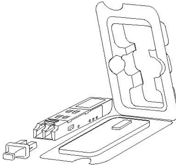
Figure 1- 17. Installing the Mini-GBIC Module
