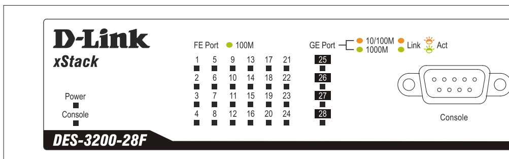
Figure 1- 4. LED Indicators on DES-3200-28F Switch
