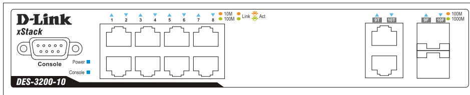
Figure 1- 5. Front Panel of the DES-3200-10
